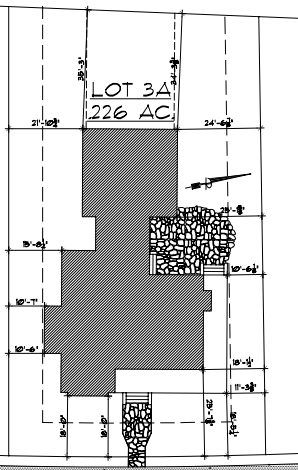
SITE PLAN
